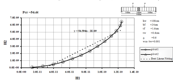
Figure (5-b) H1-H2 Relationship for the determination of critical load from Spencer technique (BCMF2, =167, \phi=0.6 )
