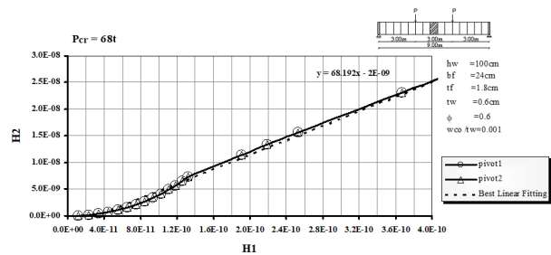
Figure (5-a) H1-H2 Relationship for the determination of critical load from Spencer technique (BCMF1, =167, \phi=0.6 )
