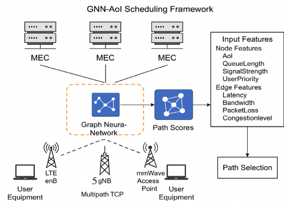
Figure 1 Proposed GNN-AoI Scheduling Framework
