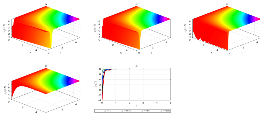
Figure 1. Graphical depiction of the nonlinear wave behavior of the exact solution showing both 3D and 2D plots corresponding to several selected values of the parameter \alpha .
