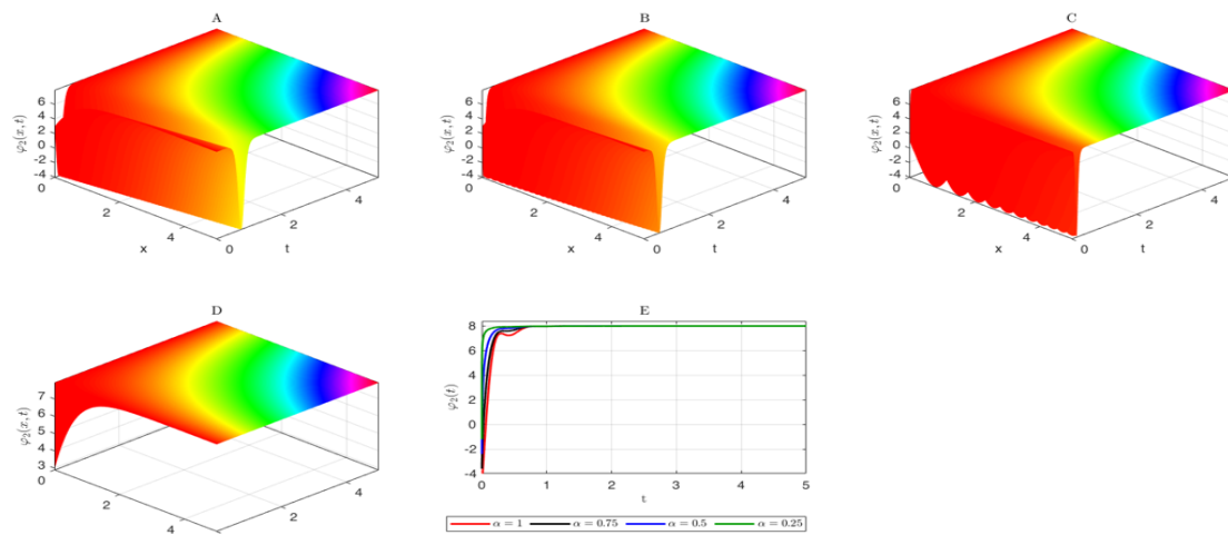
Figure 1. Graphical depiction of the nonlinear wave behavior of \varphi_1 showing both 3D and 2D plots corresponding to several selected values of the parameter \alpha .
